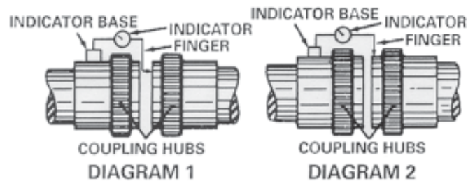
Figure 8.21 - Use of Dial Indicator to Check for Shaft Angular Alignment and Trueness
