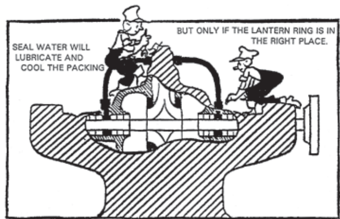
Figure 8.18 - Lantern Ring
