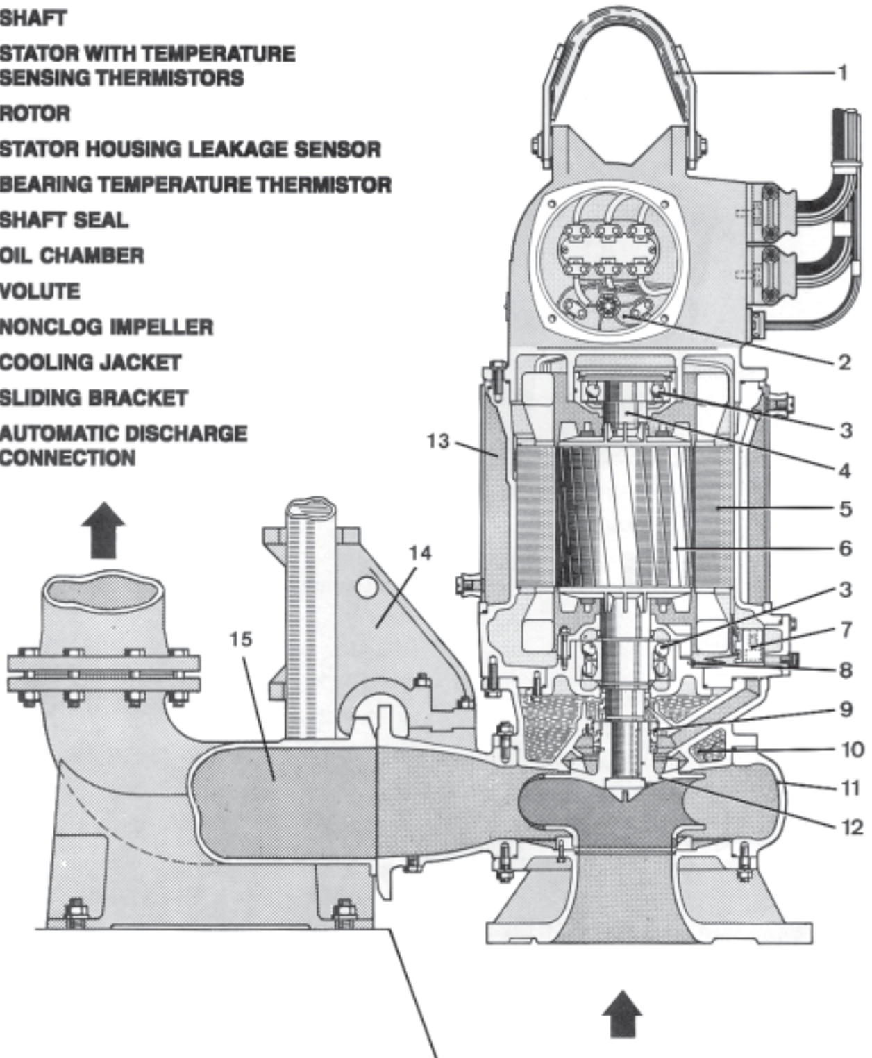
Figure 8.4 - Submersible Wastewater Pump
