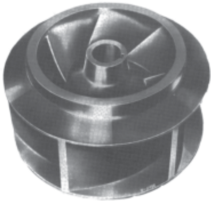
Closed Radial (Closed radial impellers are used in wastewater treatment plants.)
