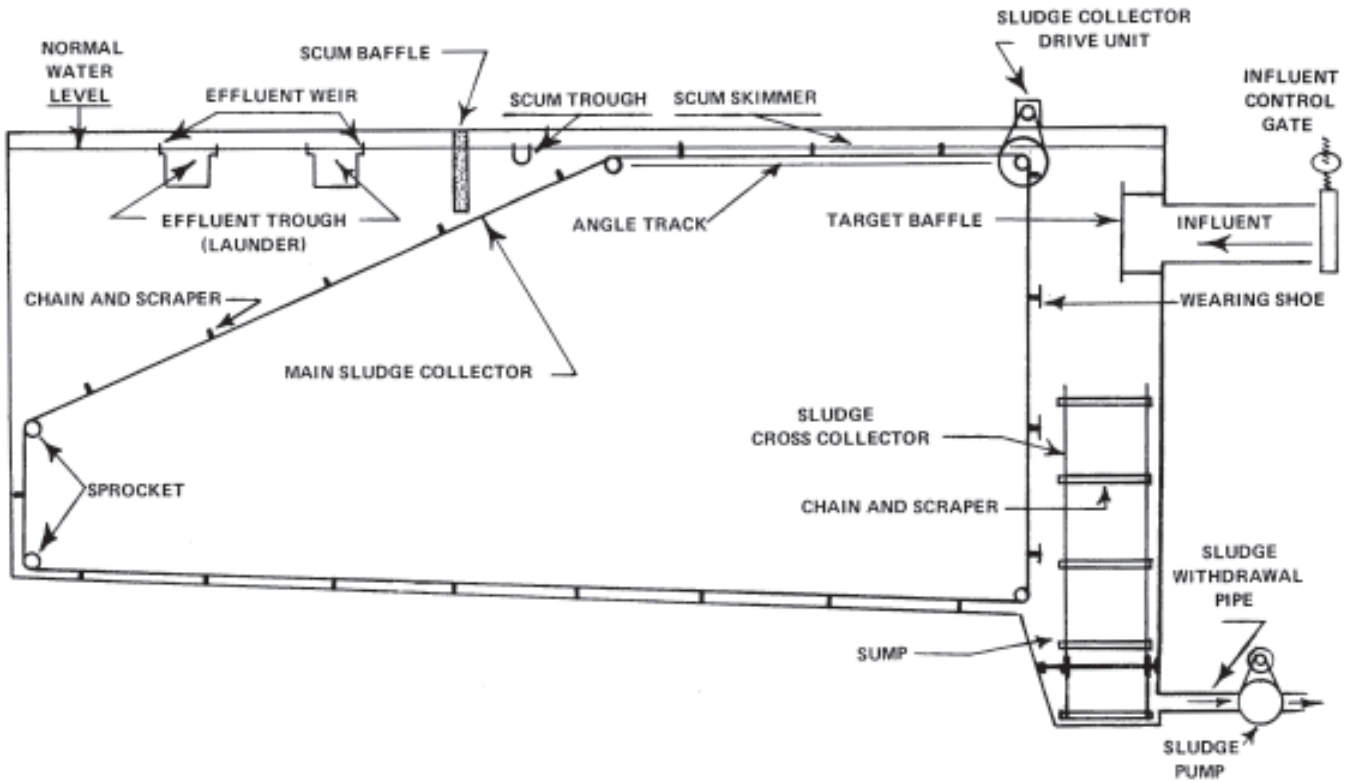
Figure 6.2 - Rectangular Sedimentation Basin
