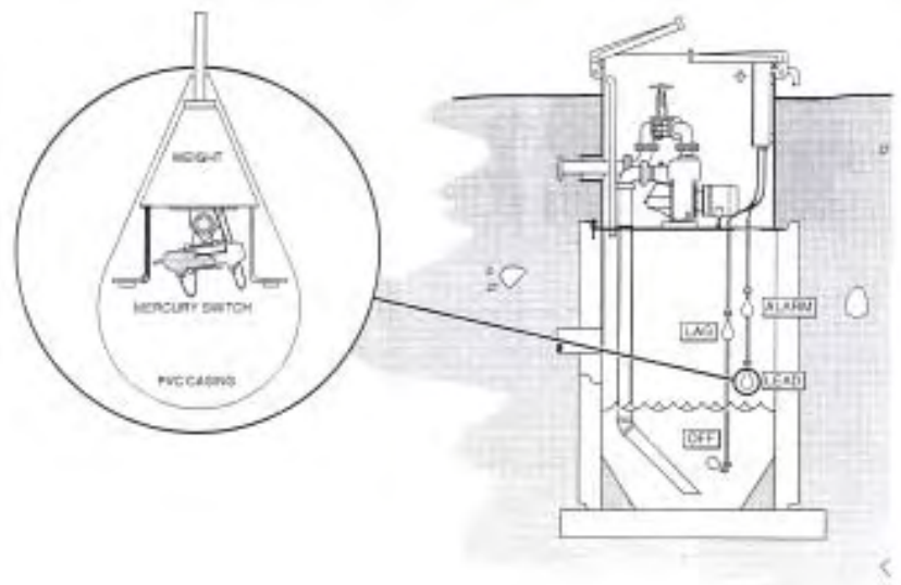
Figure 4.12 - Mercury Float Switch
