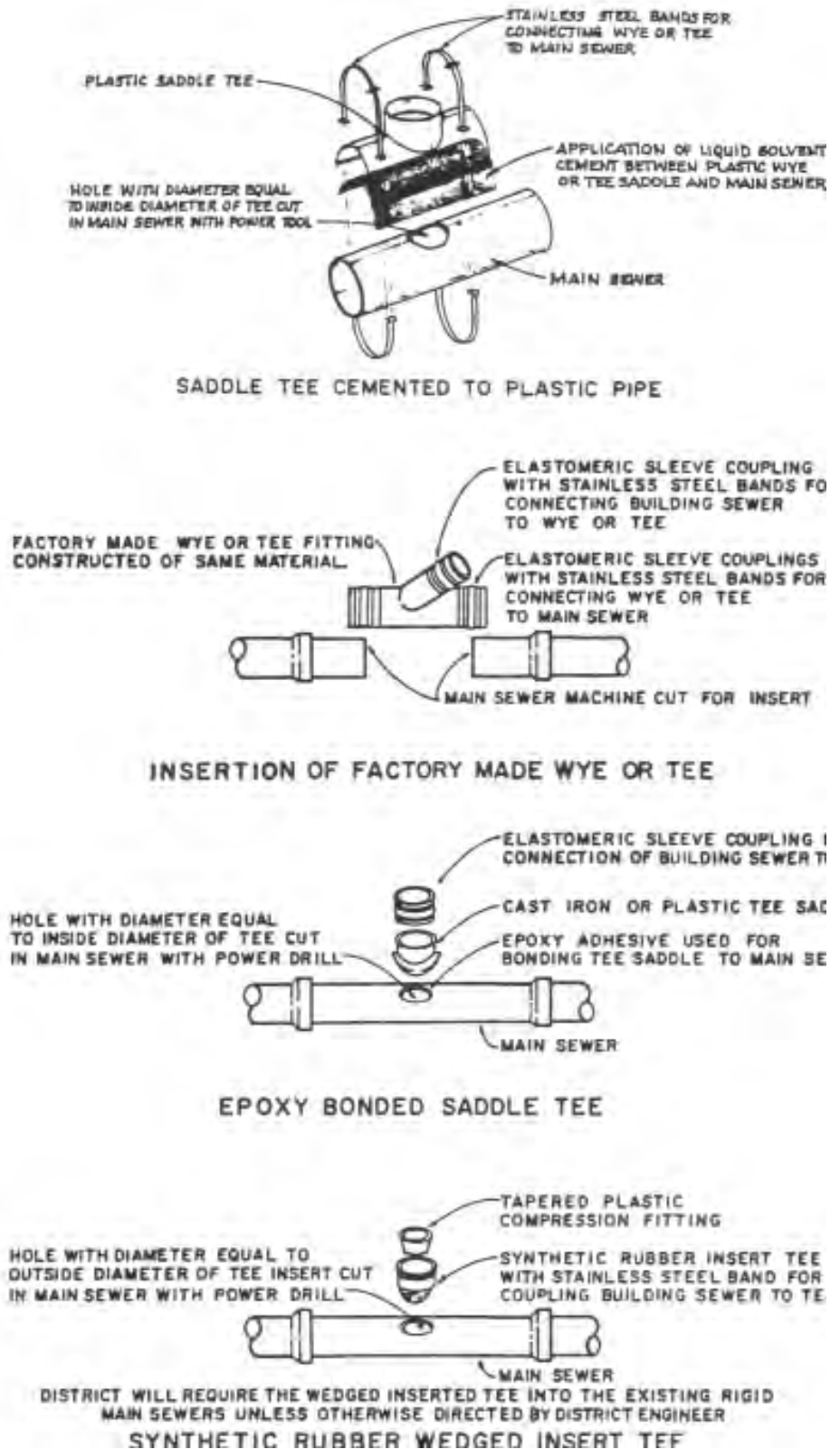
Figure 4.4 - Building Sewer Connections (taps)
