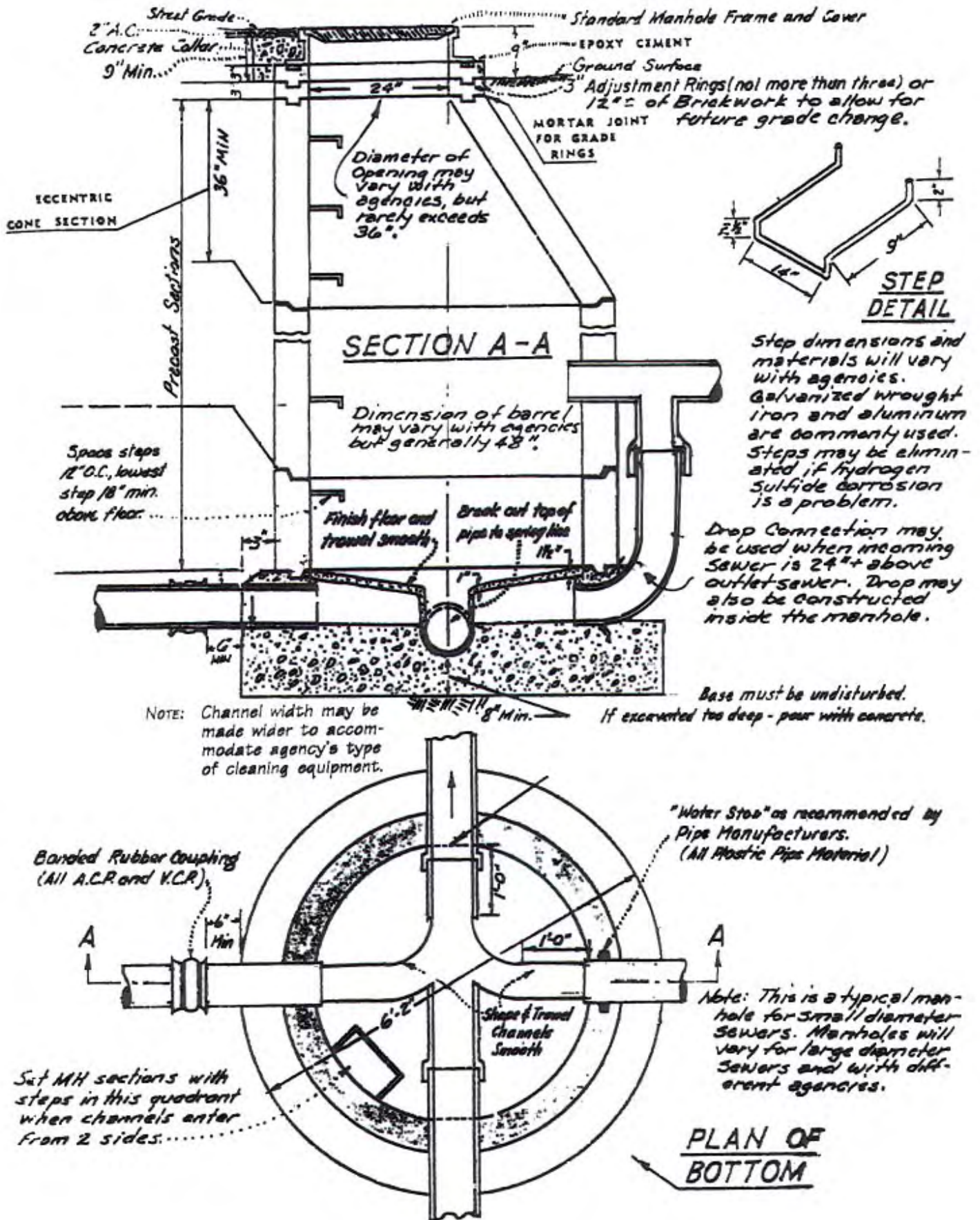
Figure 4.6 - Pre-Cast Concrete Manhole
