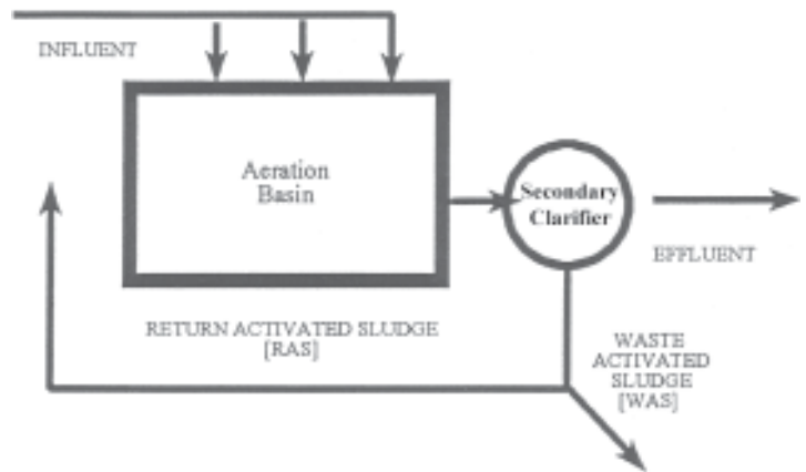
Figure 10.2 - Convention Step Feed Aeration
