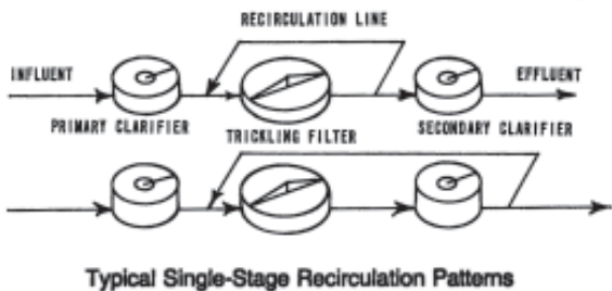
Typical Single-Stage Recirculation Patterns
