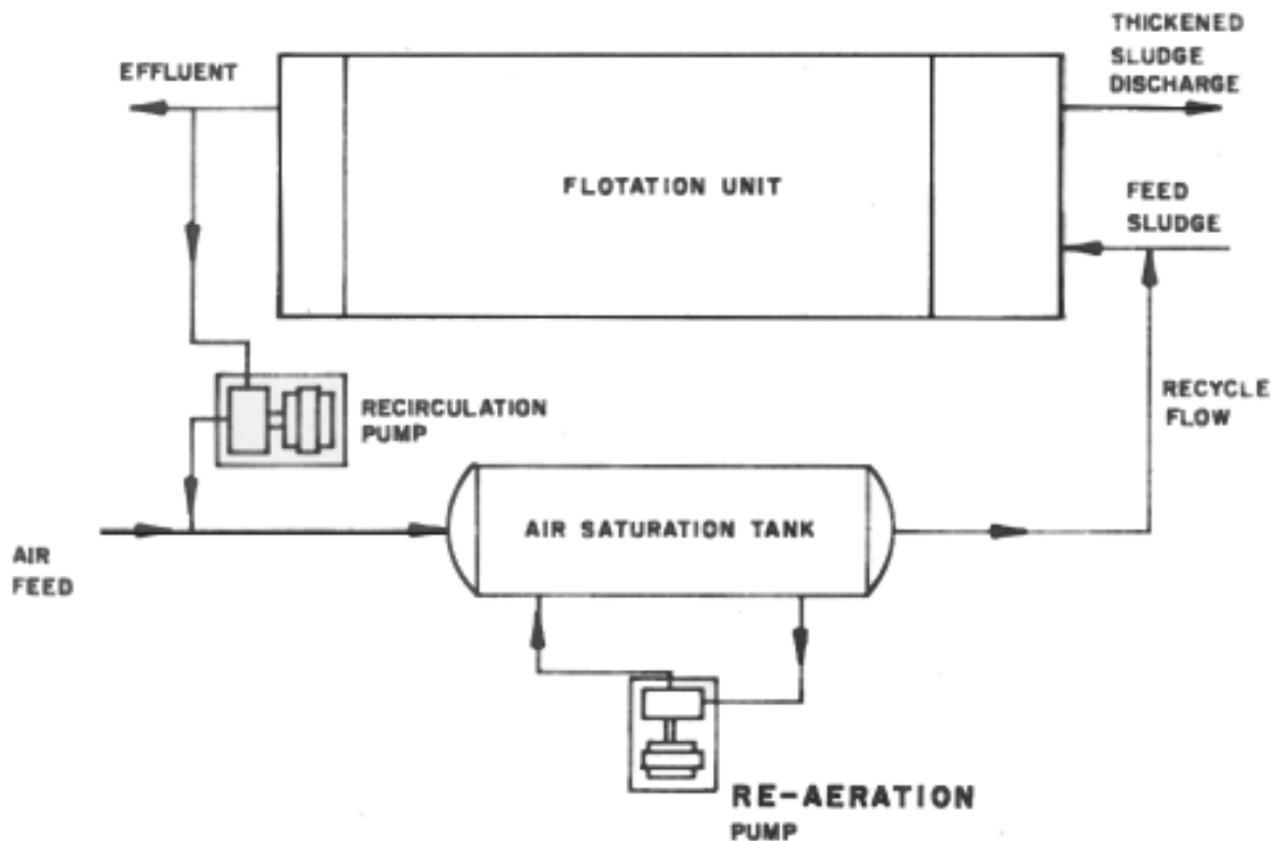
Figure 11.2 - Typical Dissolved Air Flotation (DAF) Unit
