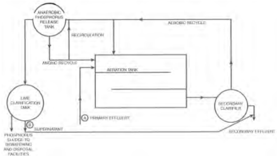
Figure 12.3 - Luxury Uptake of Phosphorus (plan flow diagram)
