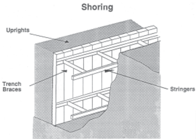
Figure 2.1 - Shoring
