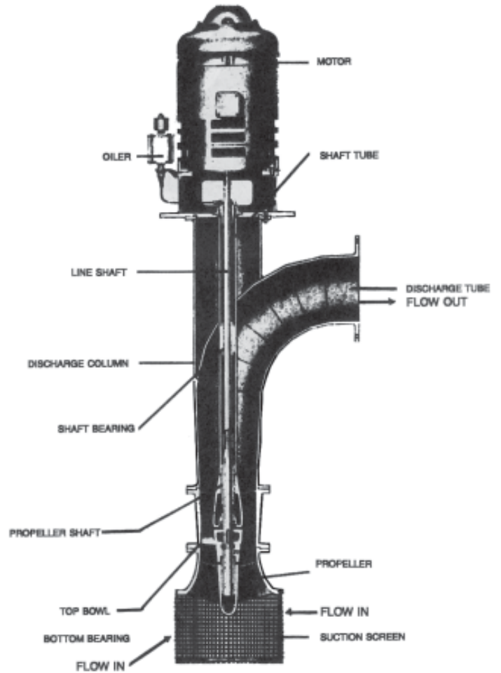
Figure 8.7 - Propeller Pump
