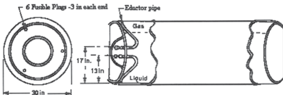
Figure 9.5 - Cross Section of a 1-ton Cylinder
