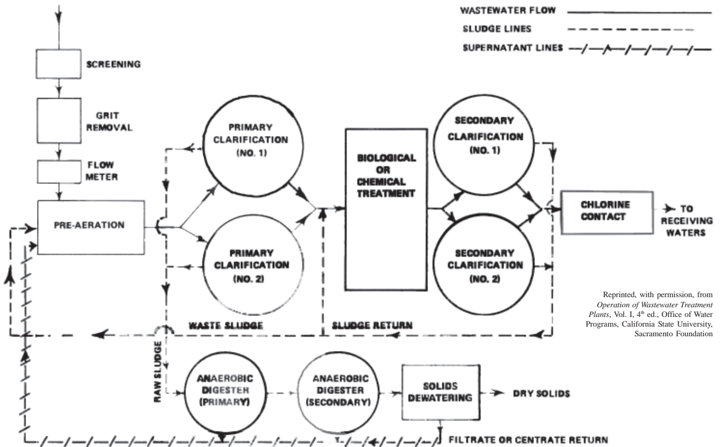
Figure 6.1 - Typical Plant Schematic
