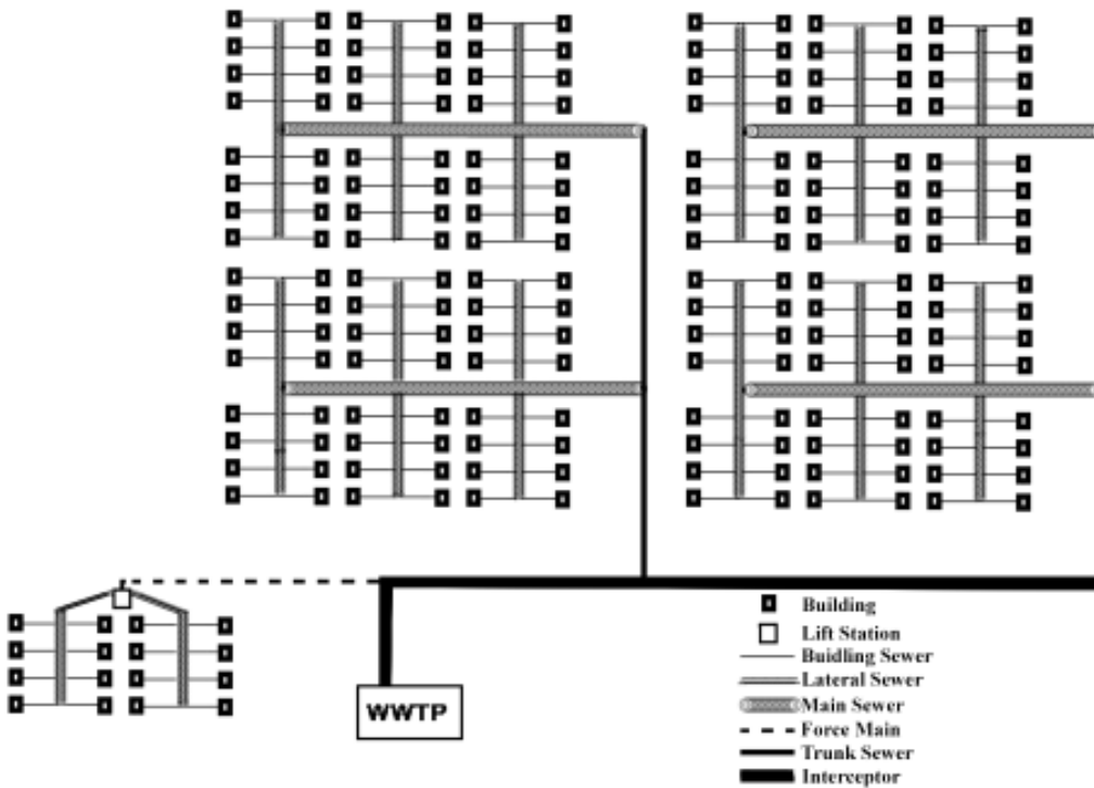
Figure 4.1 - Schematic of a Typical Gravity Wastewater Collection System
