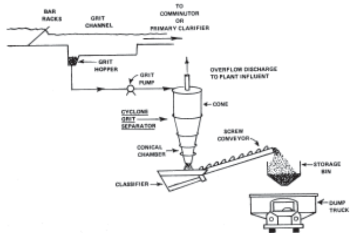
Figure 3.2 - Cyclone Grit Separator
