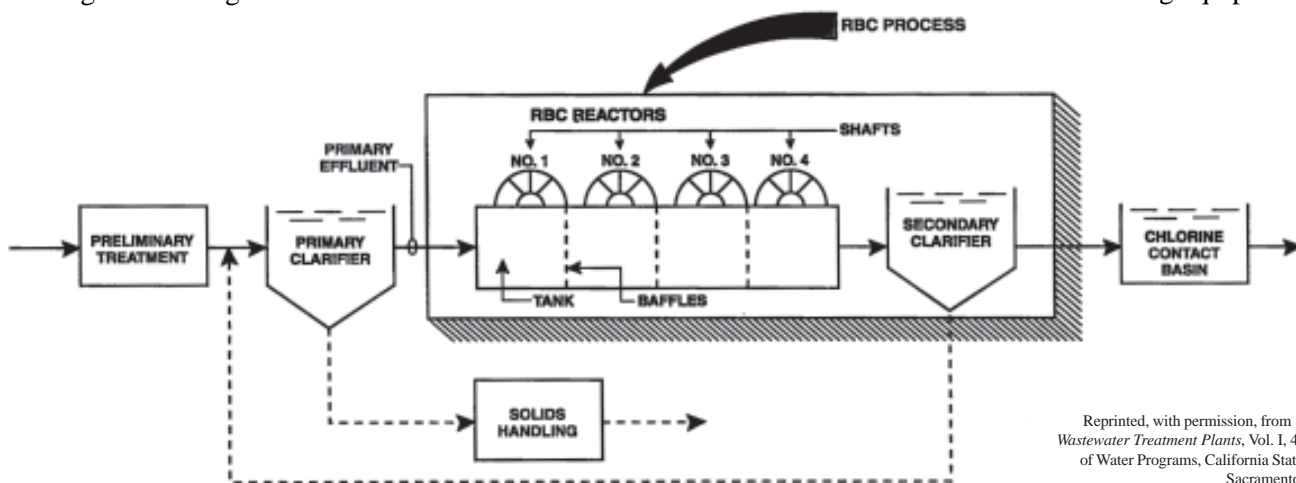
Figure 7.6 - RBC Plant Schematic
