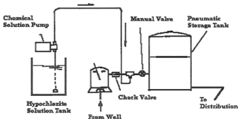
Figure 9.6 - Typical Hypochlorination System
