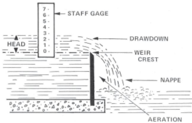
Sharp Crested Weir The staff gage is located so that "0" on the gage is the same elevation as the weir crest.
