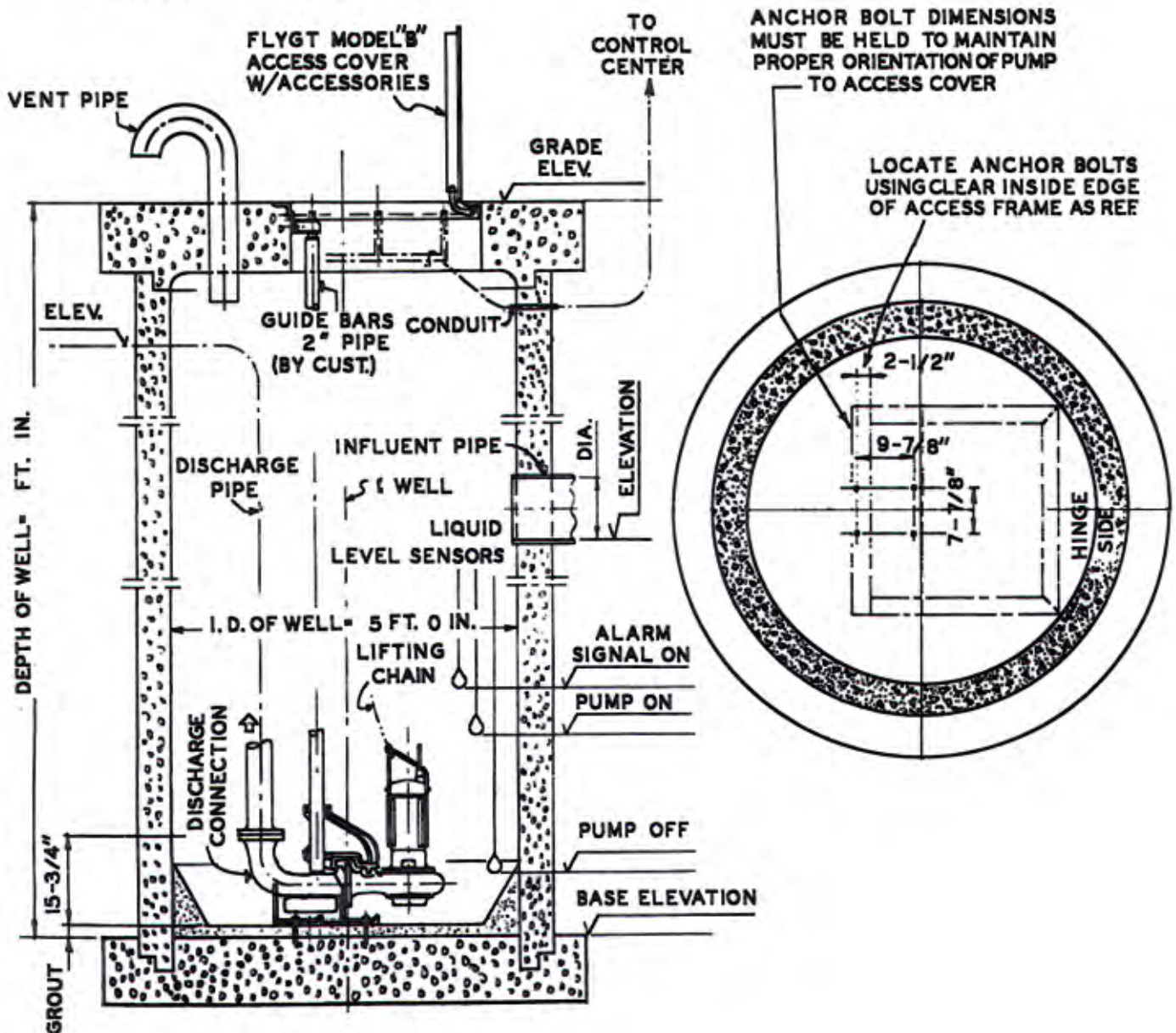
Figure 4.10 - Submersible Pump in Wet Well
