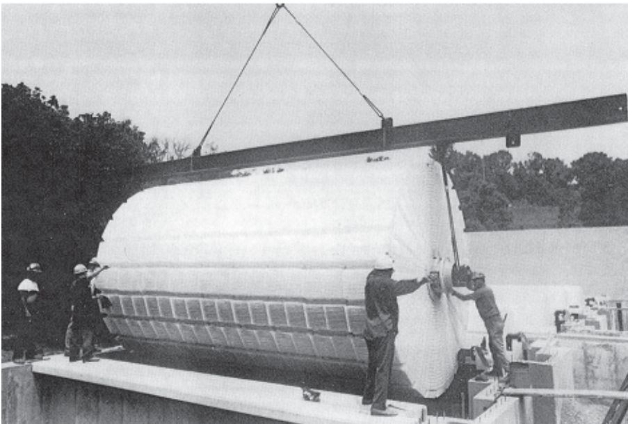
Figure 7.3 - Rotating Biological Contactor
