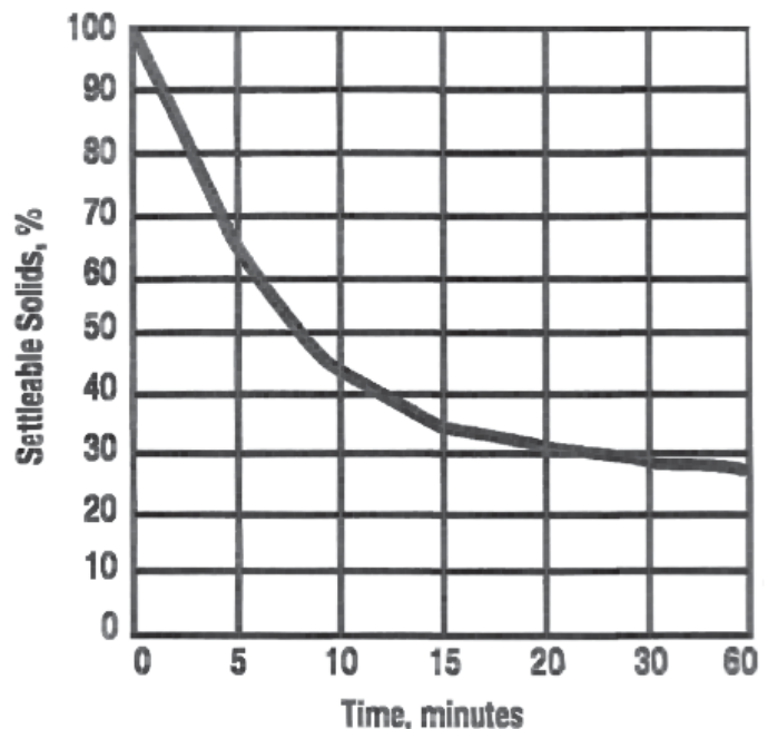
Figure 10.14 - Settleability Curve
