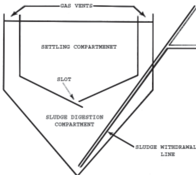
Figure 6.5 - Imhoff Tank
