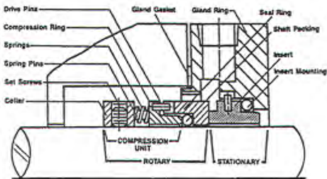
Figure 8.20 - Mechanical Seal Components
