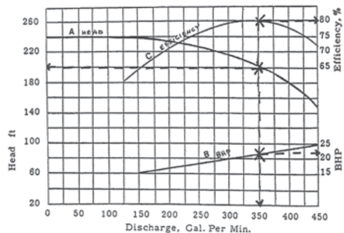
Figure 8.23 - Pump Curve
