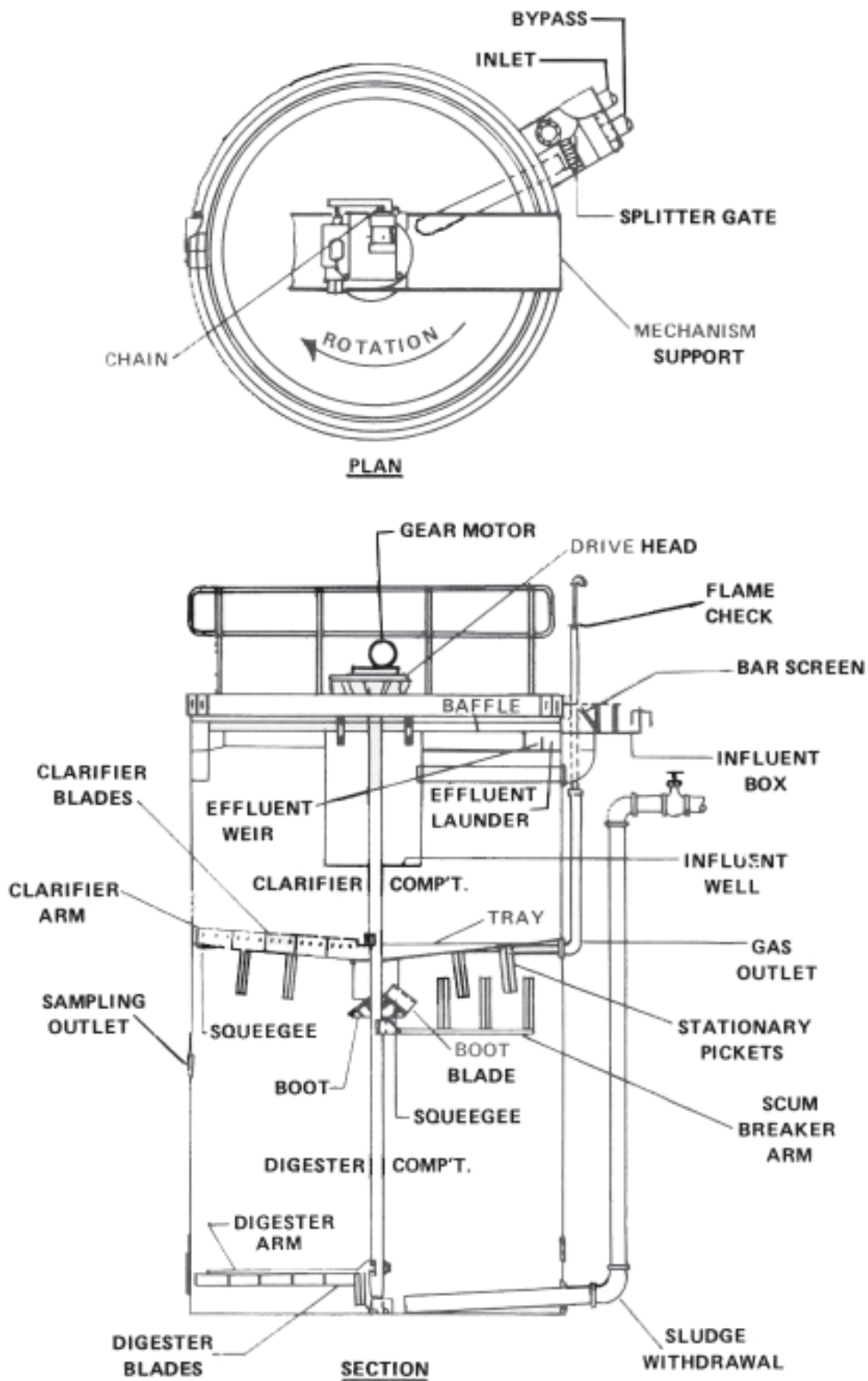
Figure 6.4 - Sedimentation Digestion Unit
