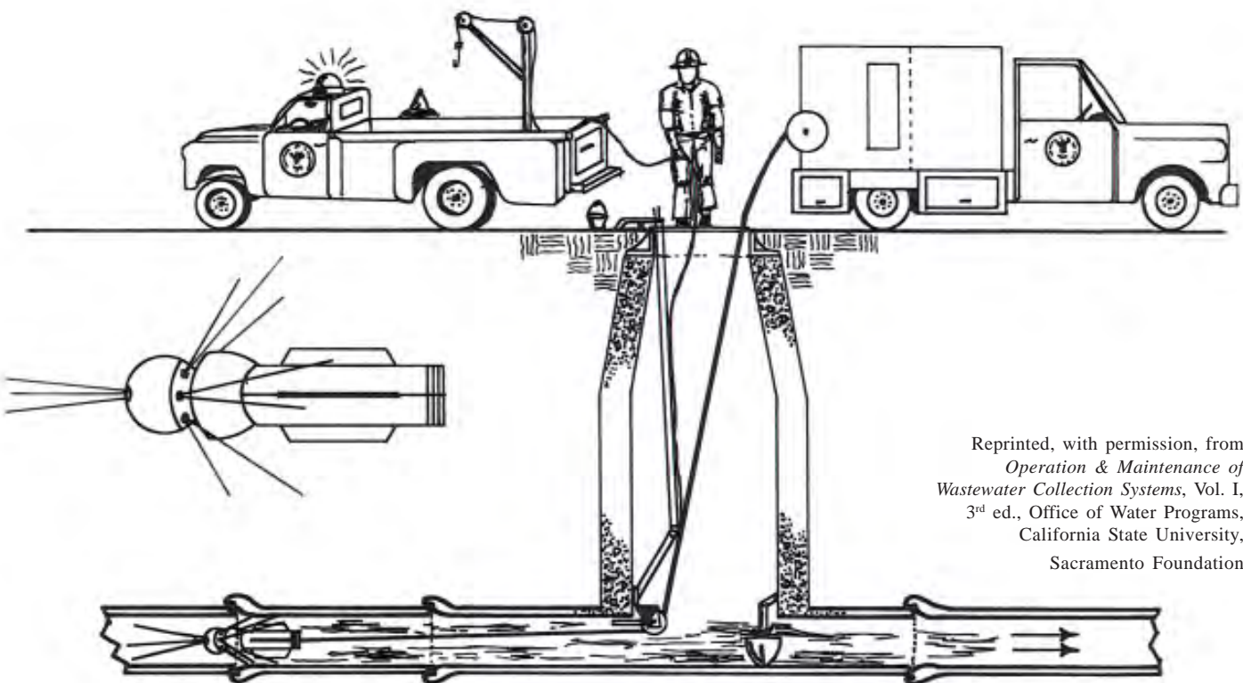
Figure 4.8 - Jet Rodder - High Velocity Cleaning Operations
