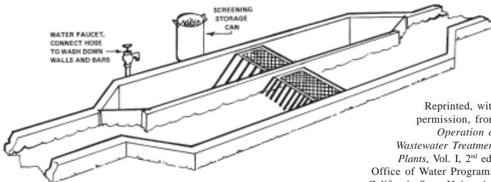
Figure 3.1 - Comminutor
