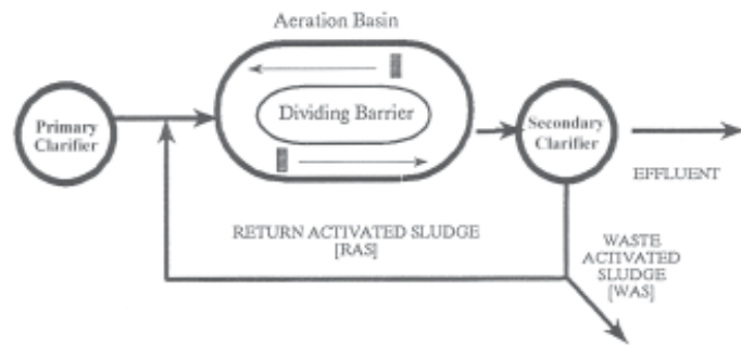
Figure 10.3 - Conventional Aeration
