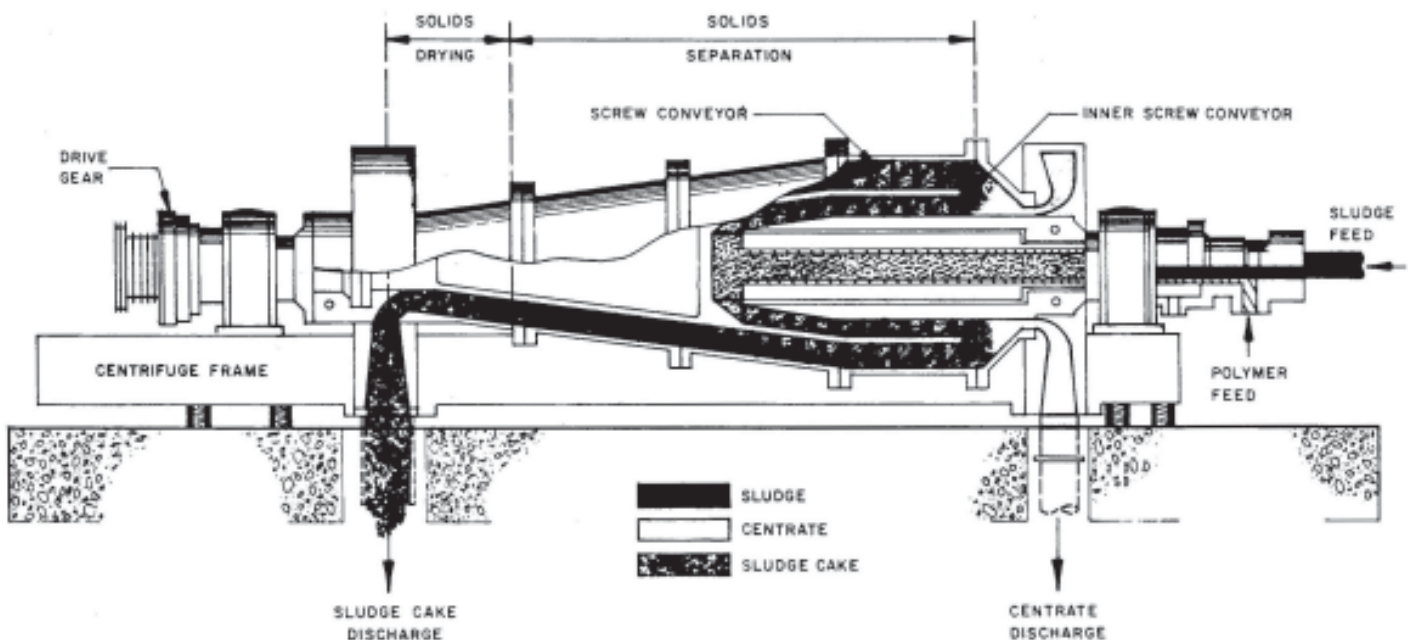
Figure 11.4 - Scroll Centrifuge
