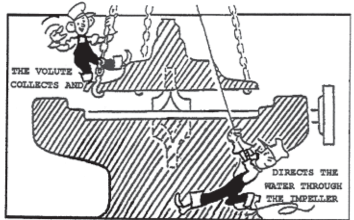
Figure 8.14 - Volute
