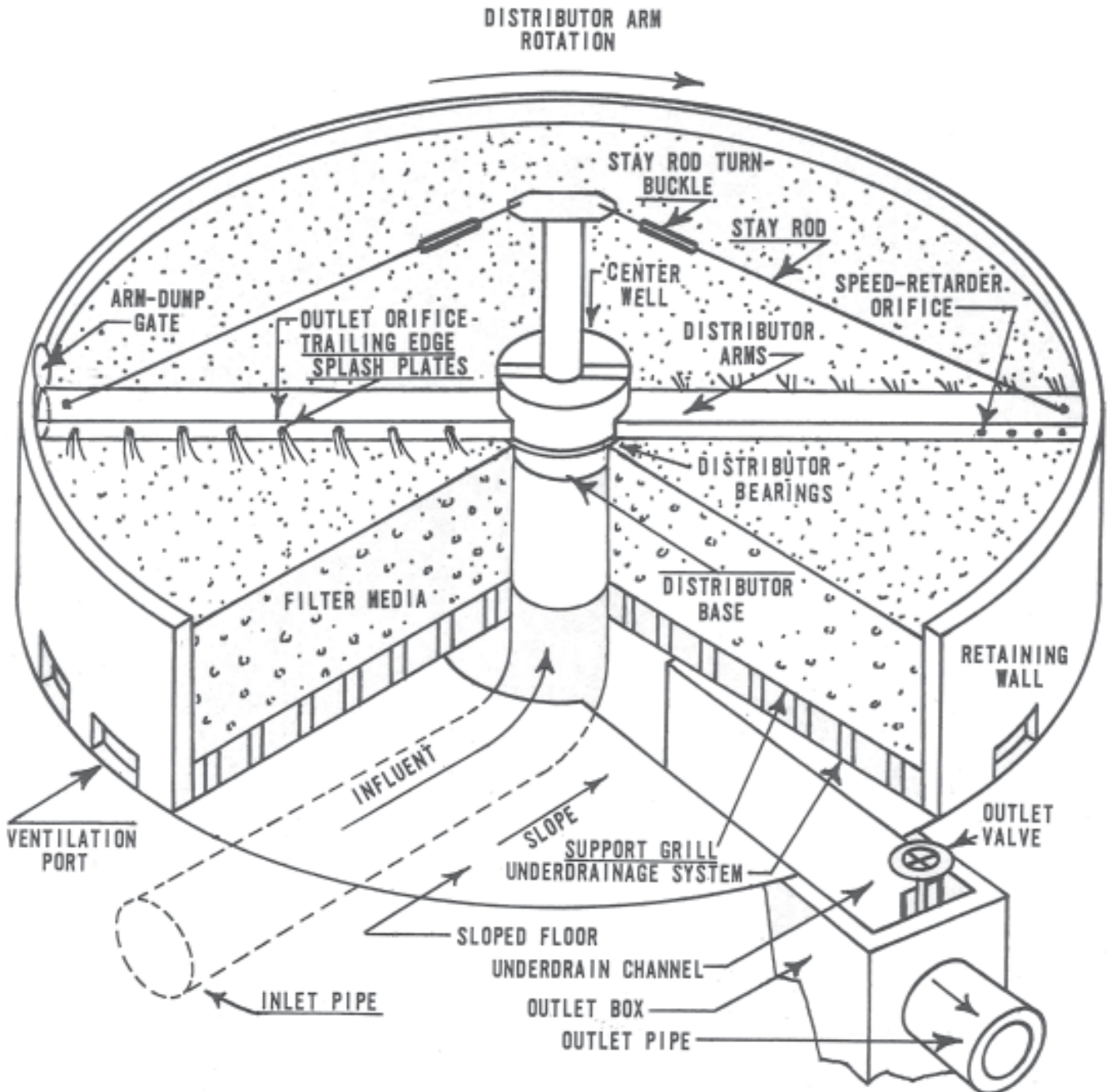
Figure 7.1 -Trickling Filter Crossection
