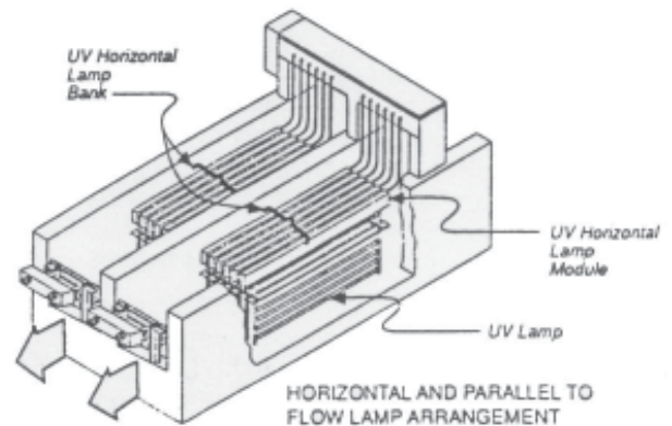
Figure 9.8 - Typical UV Lamp Configurations
