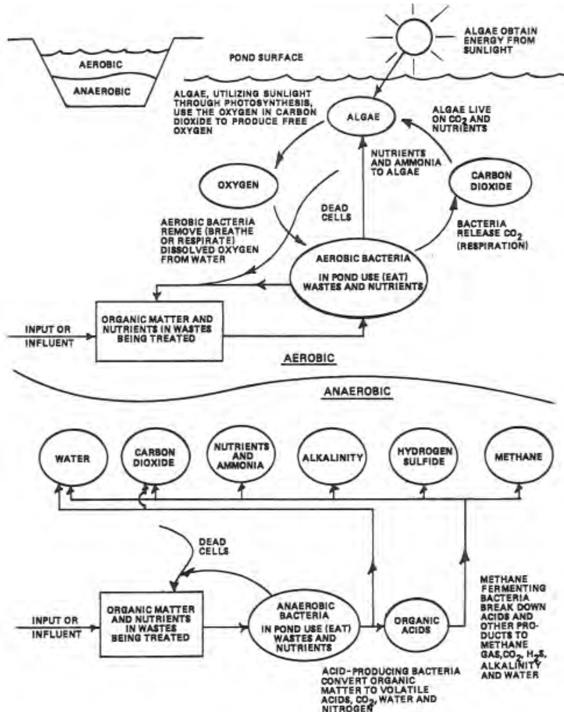
Figure 5.3 - The Role of Algae in Treating Wastes in a Pond
