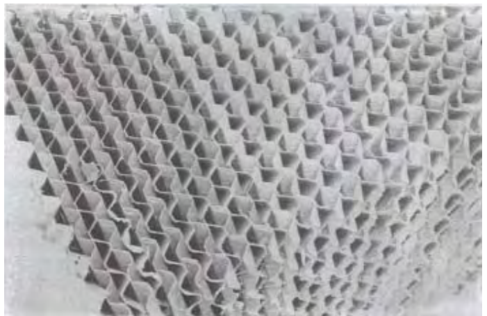
Figure 13.3 - Plastic Media Used for “Trickling Filter” Type Nitrification
