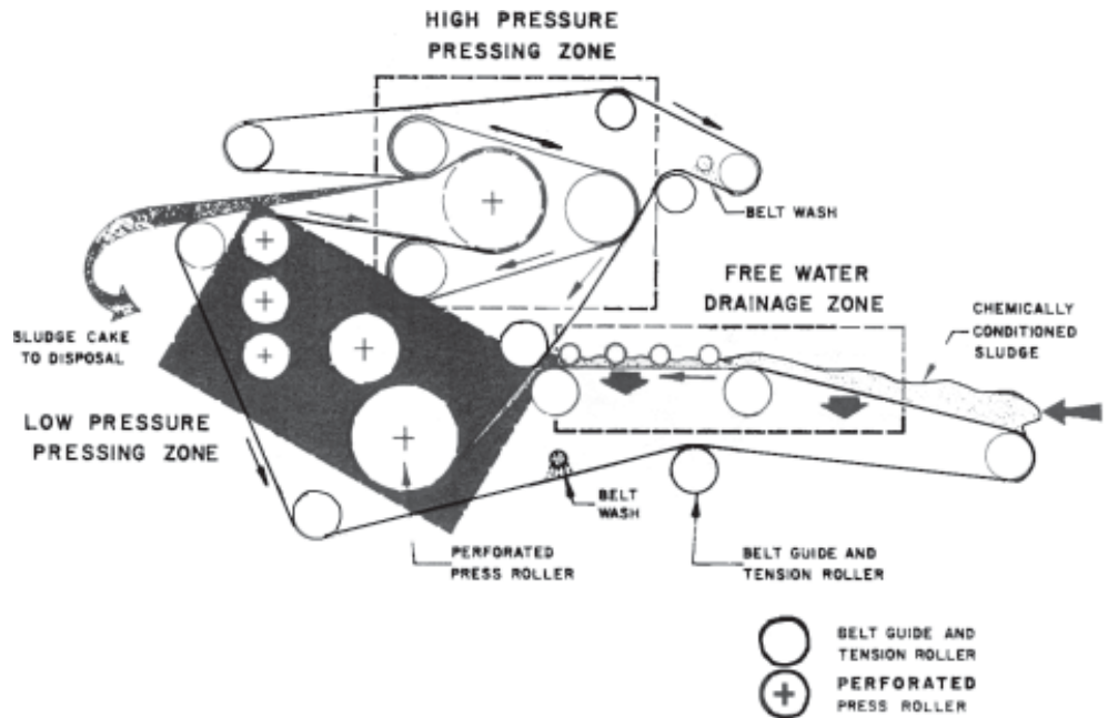
Figure 11.3 - Typical Belt Filter Press
