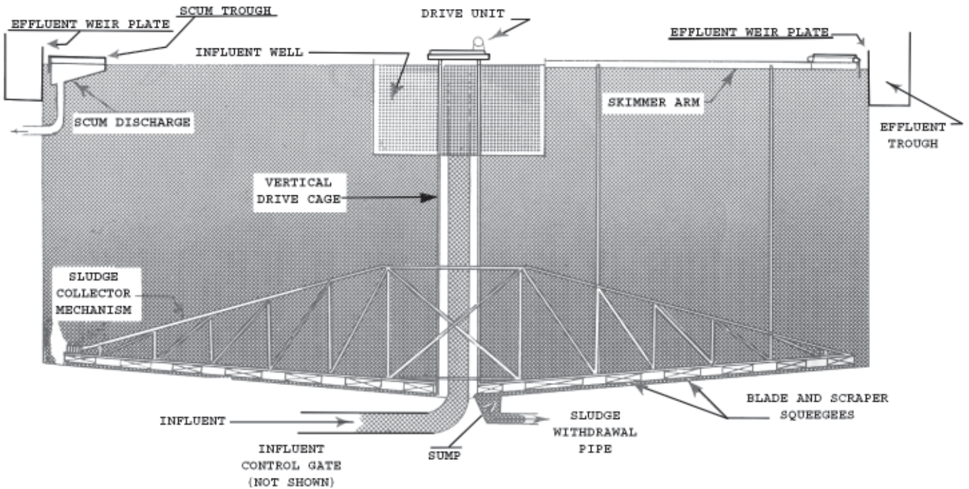
Figure 6.3 - Typical Clarifier
