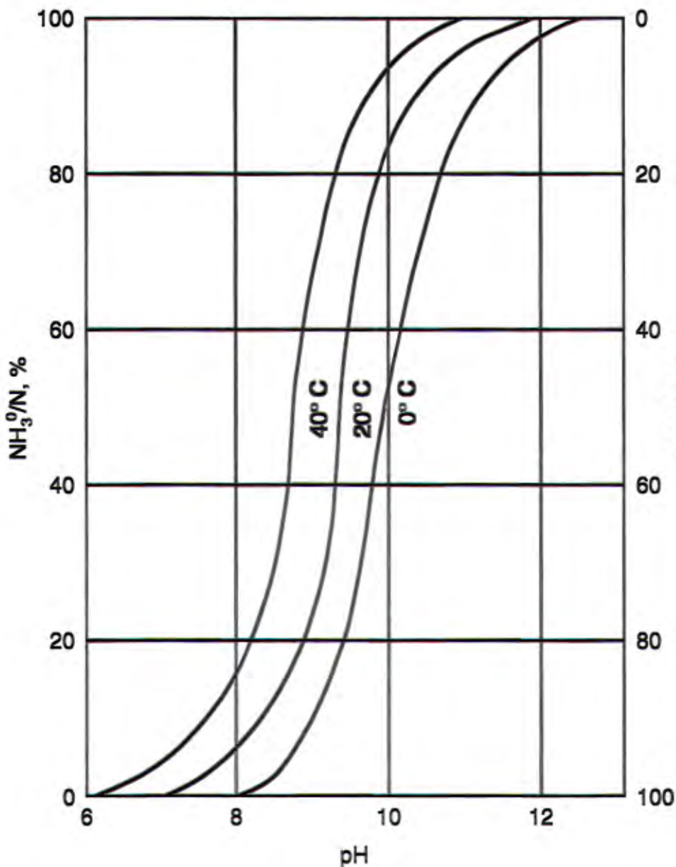
Figure 13.2 - Effects of pH and Temperature on Equilibrium Between Ammonium Ion ( NH_4^+ ) and Ammonia Gas ( NH_3^0 )
