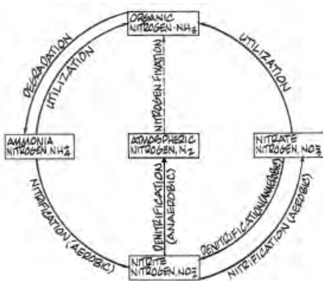
Figure 13.1 - Wastewater Nitrogen Cycle
