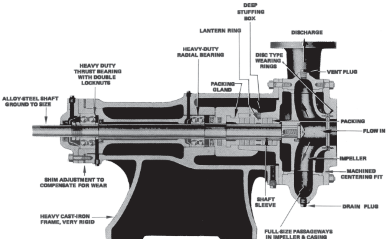
Figure 8.2 - Horizontal Nonclog Wastewater Pump with Open Impeller
