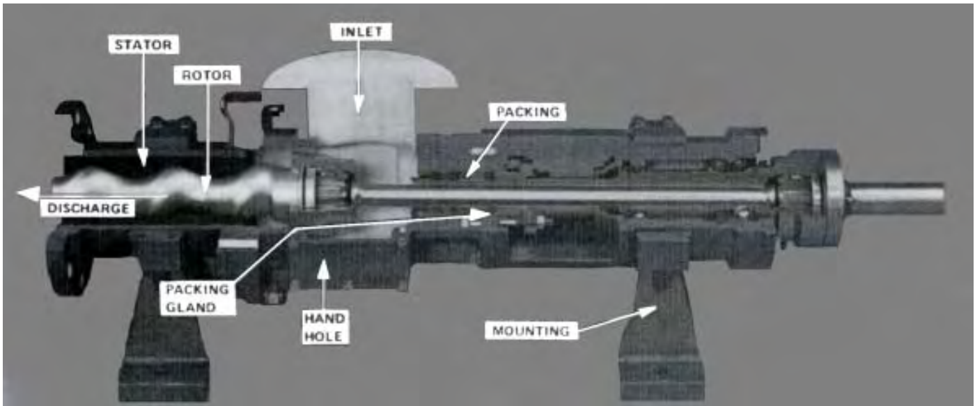
Figure 8.10 - Progressive Cavity (screw-flow) Pump
