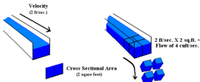
Figure 3.3 - Cross-Sectional Area of Pipe
