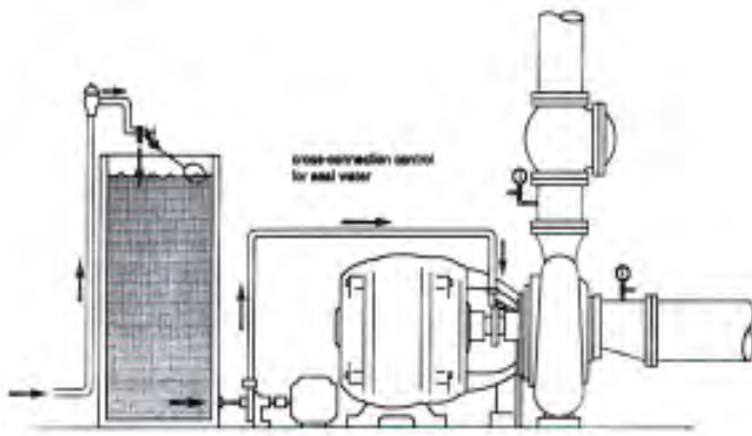
Figure 4.13 - Air Gap for Cross-Connection Control
