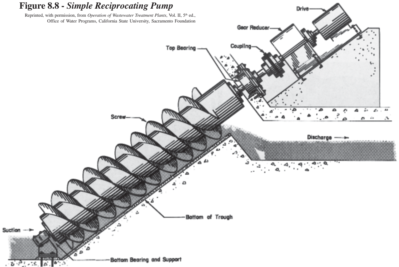
Figure 8.9 - Incline Screw Pump
