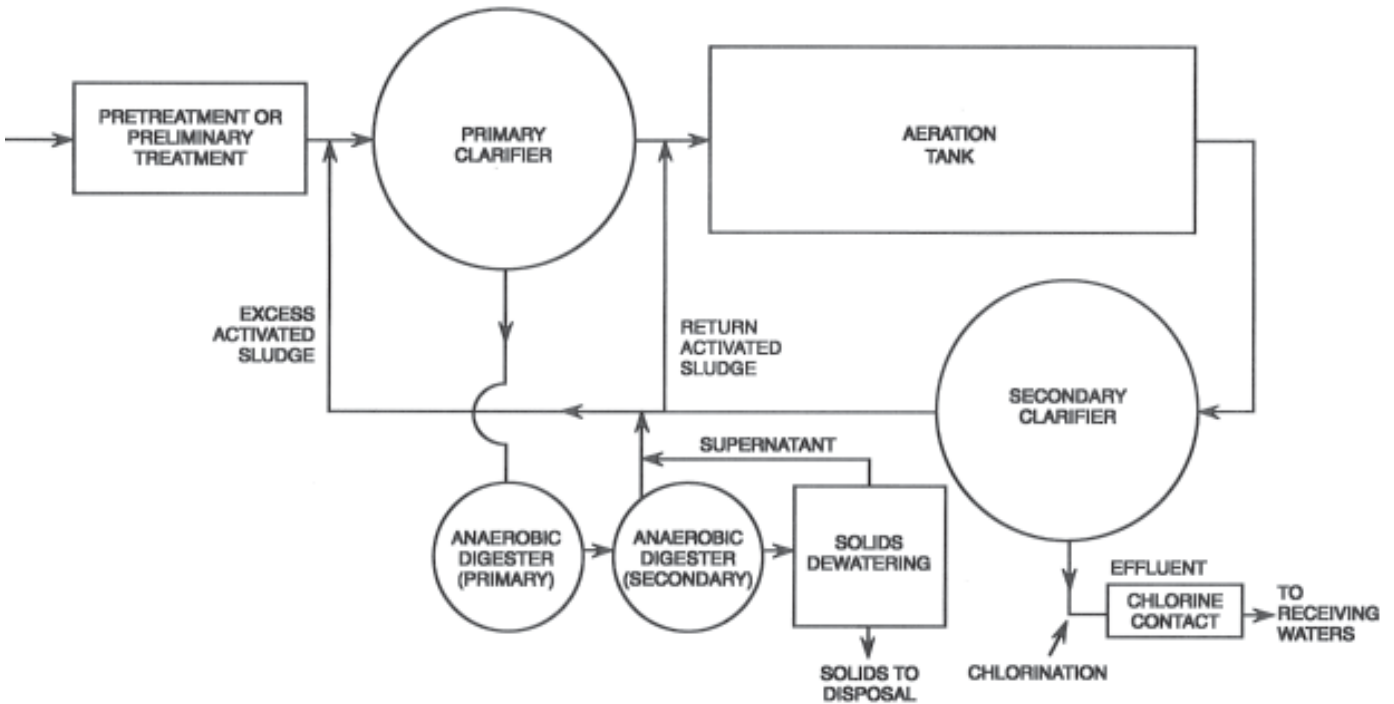
Figure 10.1 - Plant Layout
