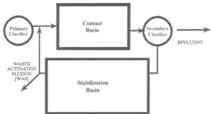
Figure 10.5 - Contact Stabilization
