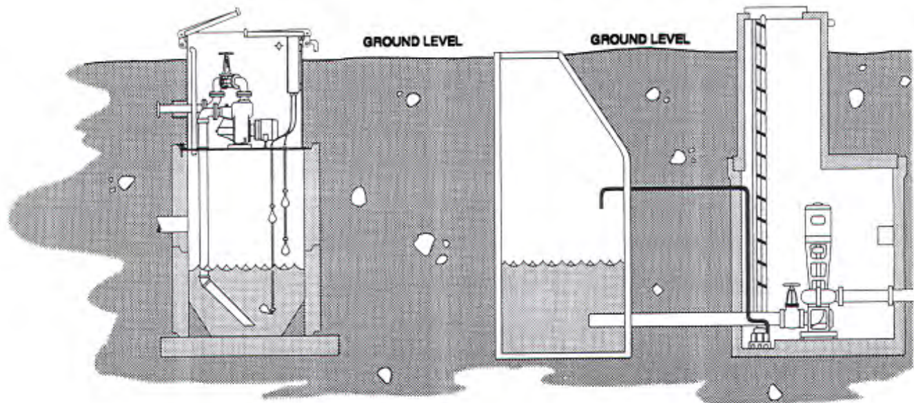
Dry Well Lift Station
