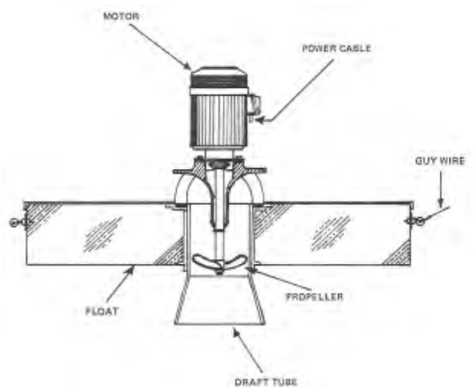
Figure 5.4 - Surface Aerator
