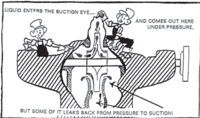
Figure 8.16 - Recirculation through the Impeller
