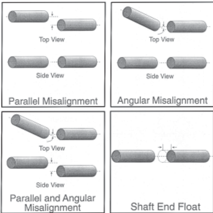
Figure 8.22 - Types of Shaft Misalignment and End Float
