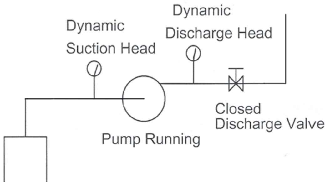
Figure 8.24 - Shut Off Head
