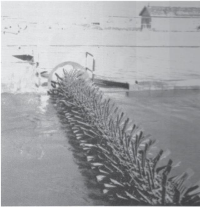
Figure 10.7 - Brush Rotor
