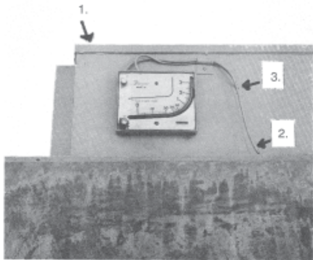
Manometer on a filter chamber (not a U-tube manometer) reading inches of pressure difference
