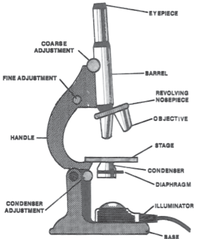
Figure 10.19 - Schematic of a Compound Light Microscope with Built-in Light Source
