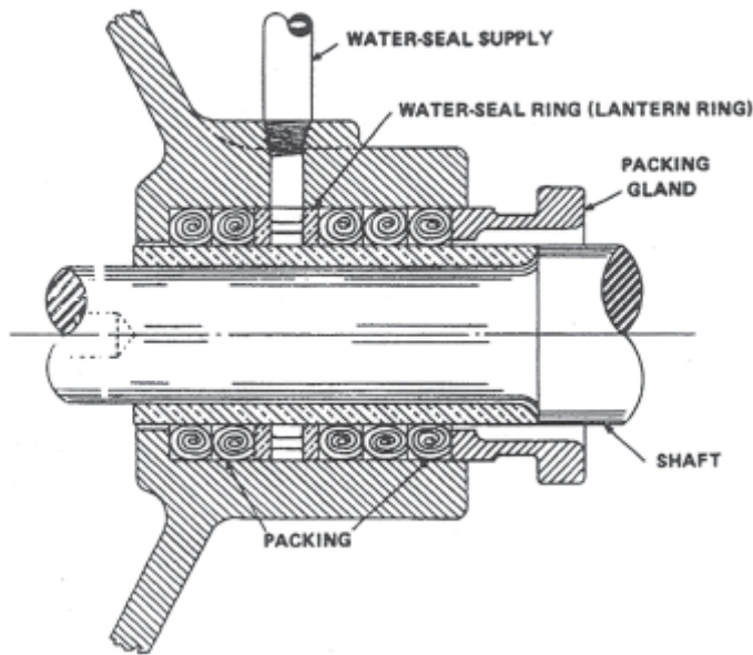
Figure 8.19 - Stuffing Box with Lantern Ring
