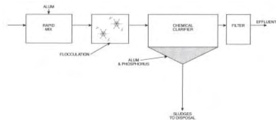
Figure 12.4 - Alum Flocculation as used in a Clarification Process
