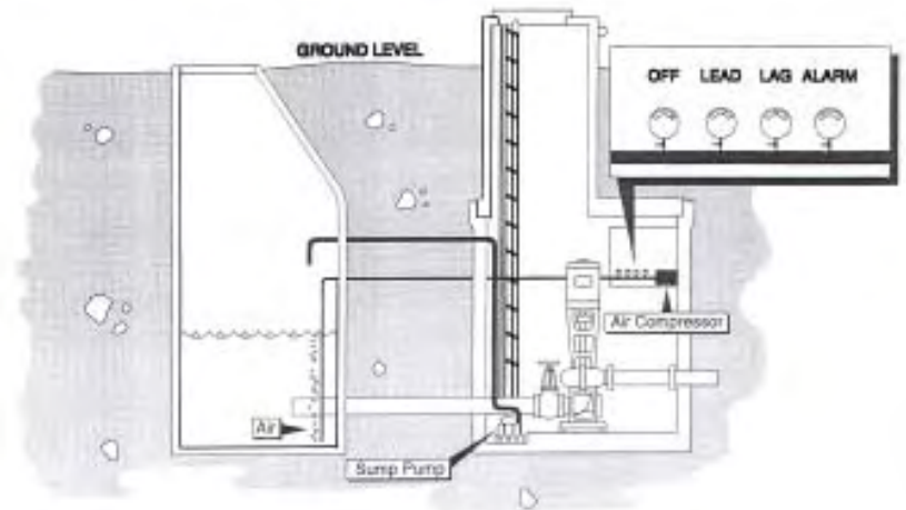
Figure 4.11 - Pneumatic Controllers
