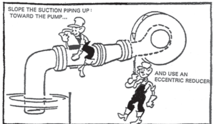
Figure 8.15 - Suction Piping Installation
