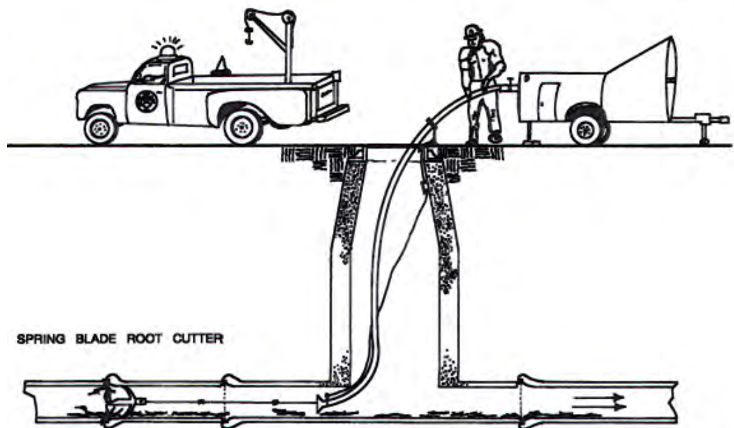
Figure 4.5 - Power Rodder Operation
