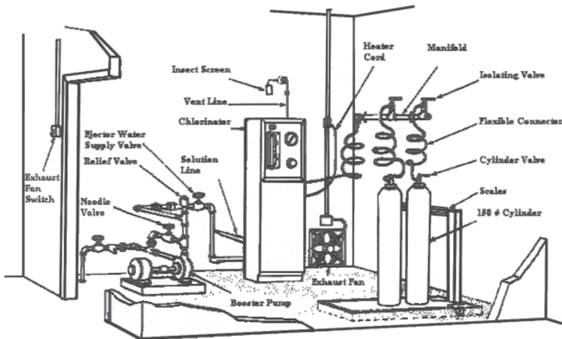
Figure 9.3 - Gas Chlorination Installation (150 Lb. Cylinders)
