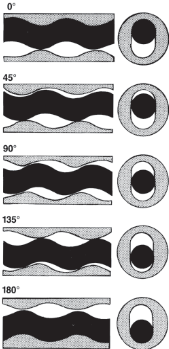
Figure 8.11 - Pumping Principle of a Progressive Cavity Pump
