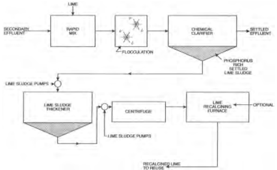
Figure 12.1 - Lime Precipitation Process
