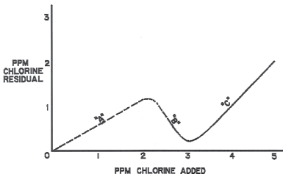
Figure 9.1 - Breakpoint Chlorination Curve
