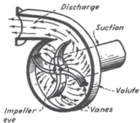
Figure 8.1 - Centrifugal Pump Crosssection
