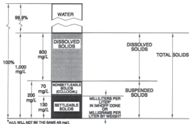
Figure 1.5 - Typical Solids in Domestic Raw Wastewater
