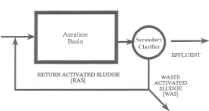
Figure 10.4 - Extended Aeration
