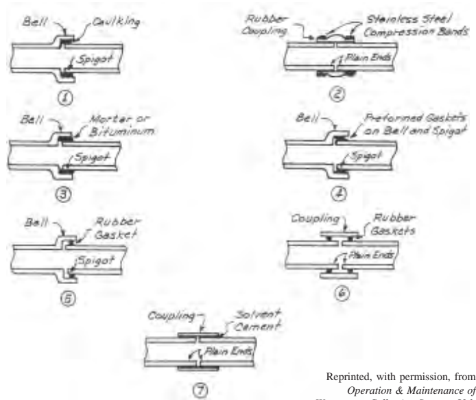
Figure 4.2 - Types of Joints
