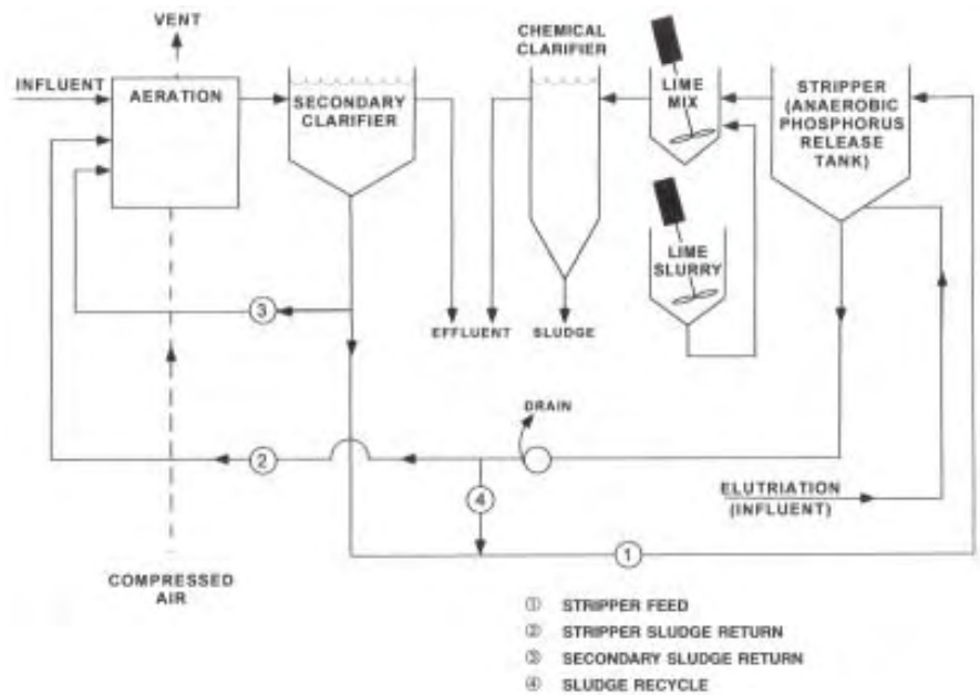
Figure 12.2 - Luxury Uptake of Phosphorus (elevation flow diagram)
